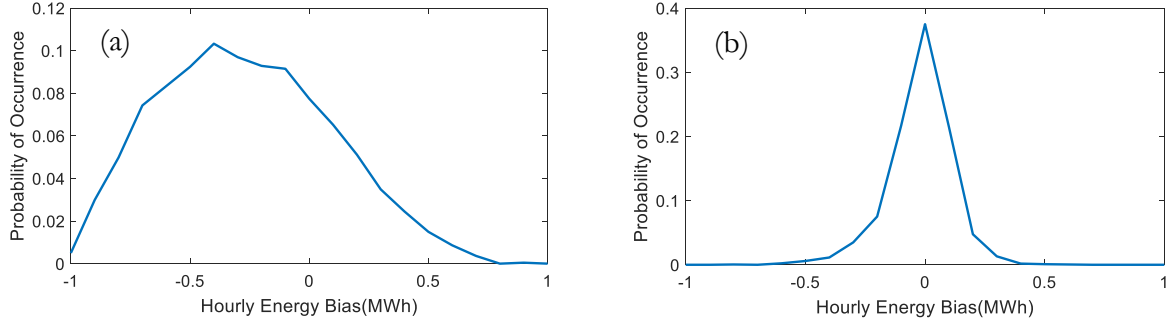
Figure 6.6.5. (a) PDF of PJM RegA hourly energy bias during June–August 2017; (b) PDF of PJM RegD hourly energy bias during June–August 2017.
